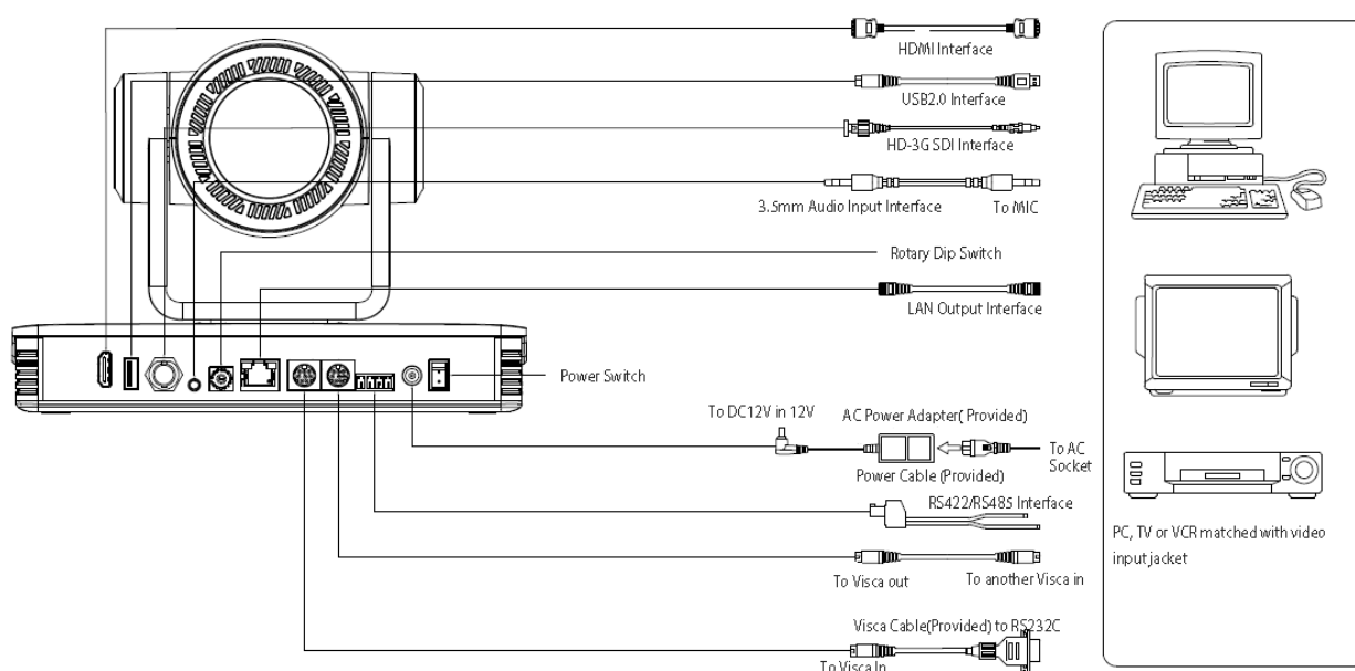
Figure2-2 Interface Diagram
