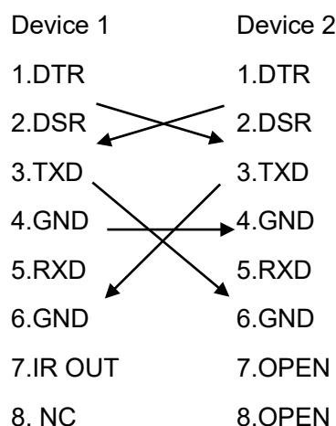
Figure2-4 VISCA Networking Diagram
