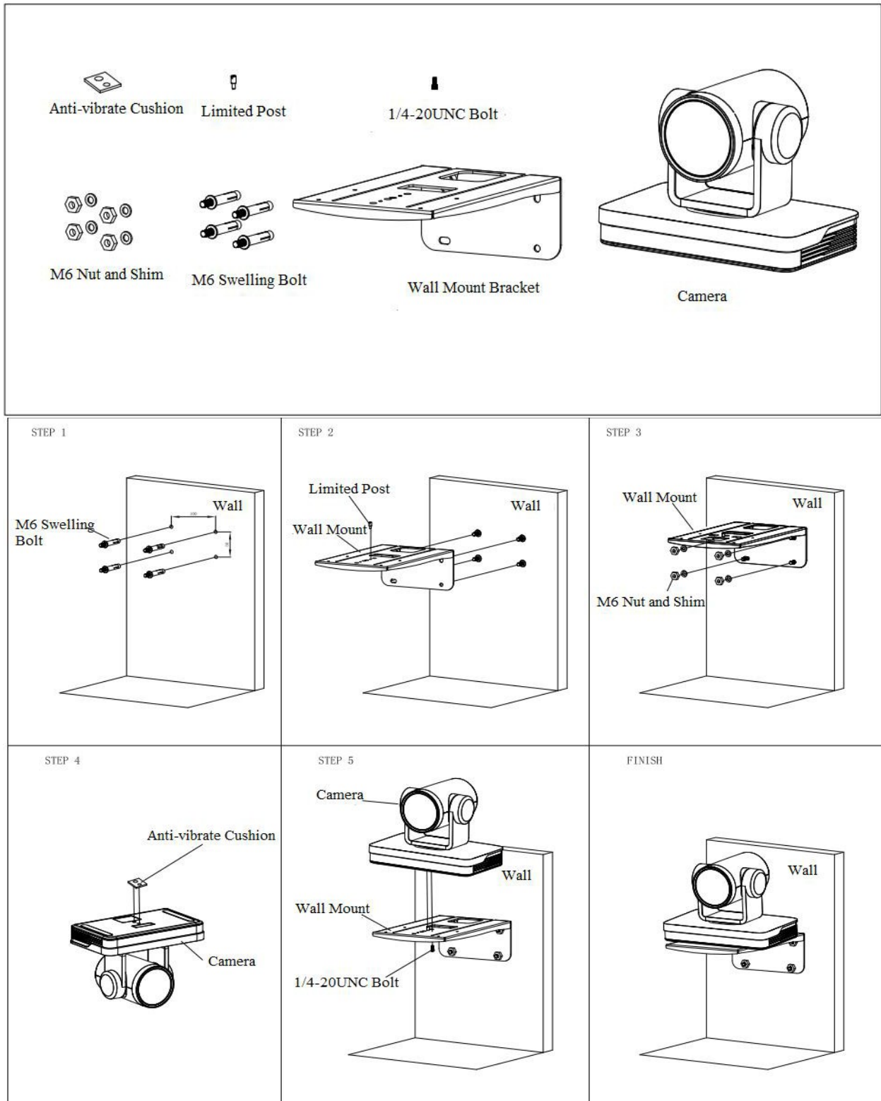
Figure1-2 Steps of Wall Mount
