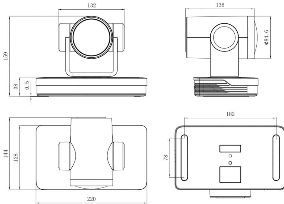
Figure2-1 Product Dimension
